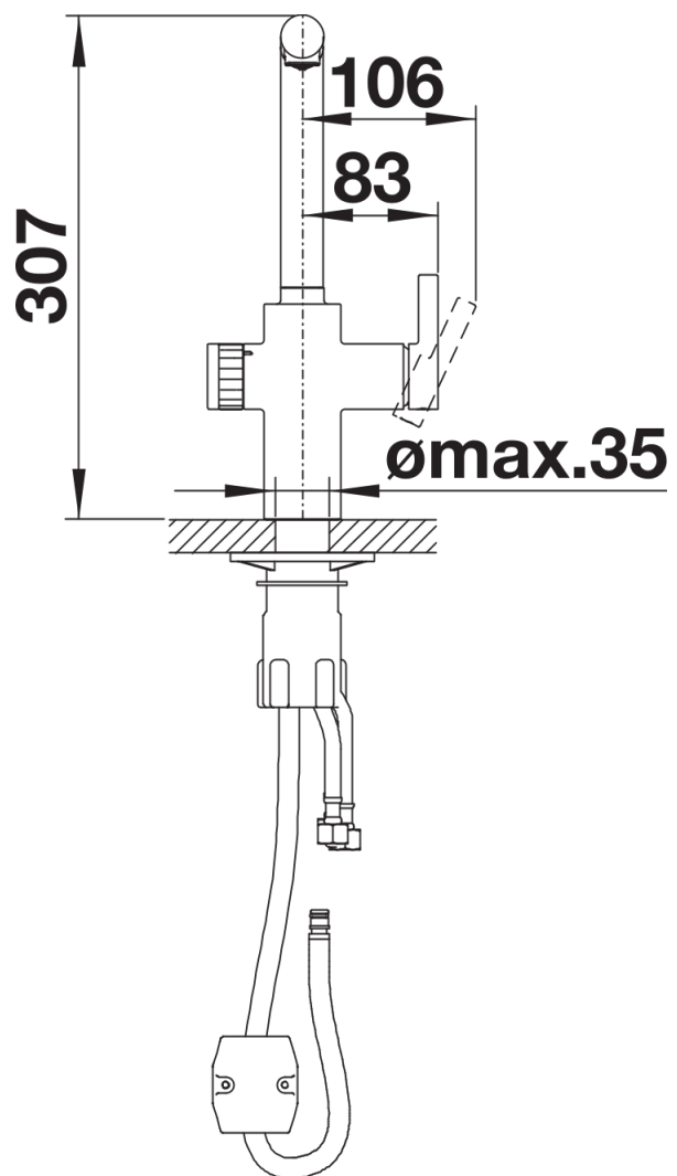
Side view hand gear 2D
